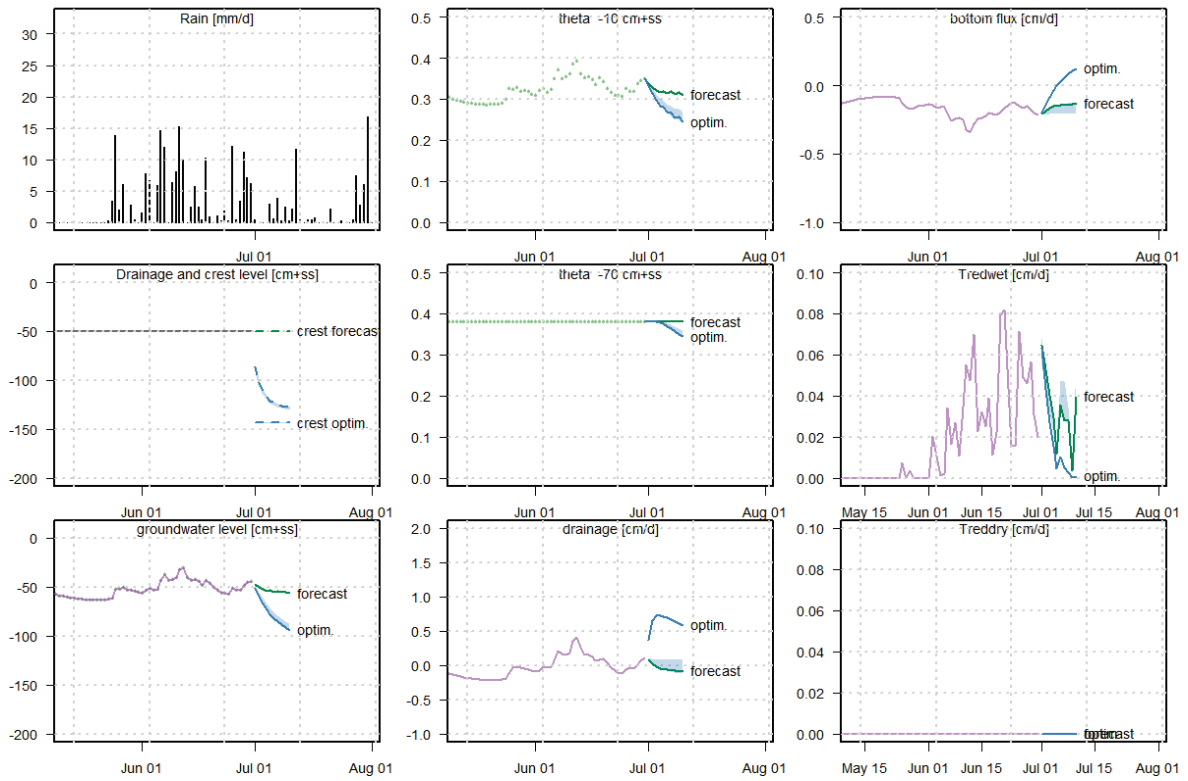
Figure 20: Example of forecast and optimization of the crest level for wet conditions. In order to limit future oxygen stress (Tredwet, forecast), the crest level needs to be lowered (crest optim., see also Figure 18). This will increase the drainage flux, lower the groundwater level and soil moisture contents (theta), and limit Tredwet..
