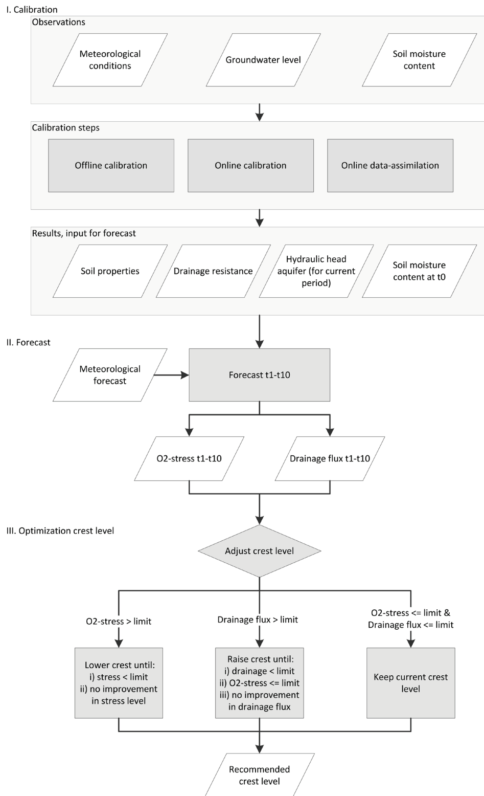
Figure 4: Estimation of the recommended crest level, based on observed groundwater levels and soil moisture conditions, process-based model simulations, and 10-day weather forecasts.
