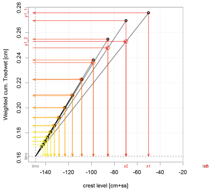
Figure 18: Optimization routine, if \Sigma weighted Tredwet > limit. First, the lowest possible stress level (limy, see y-axis) is calculated, by running SWAP with the lowest possible crest level (limx, see x-axis). Then, the next crest level is derived by i) calculate y-value by a fraction of the difference between y1\_1 (the current weighted cumulative Tredwet) and limy: y1\_2 = limy + factor * abs(y1\_1 - limy) , ii) calculate next x value from a linear relationship between (x1, y1\_1) and (x2, y1\_2) , iii) run swap with this x value, which gives a new yn\_1 value. This procedure is repeated until: abs(y1\_1 - limy) < 1e-3 (i.e. very small absolute difference) or abs(y1\_1 - limy) \leq myfactor2 * limy (i.e. very small relative difference with lowest possible value) or y1\_1 \leq limy.accept (i.e. very small difference with accepted value) or x1\_2 < minx or x1\_2 > maxx ) (i.e. next estimate of crest level below lowest or above highest possible crest level) or nrow(it.out) > 100 (i.e. too many iterations)
