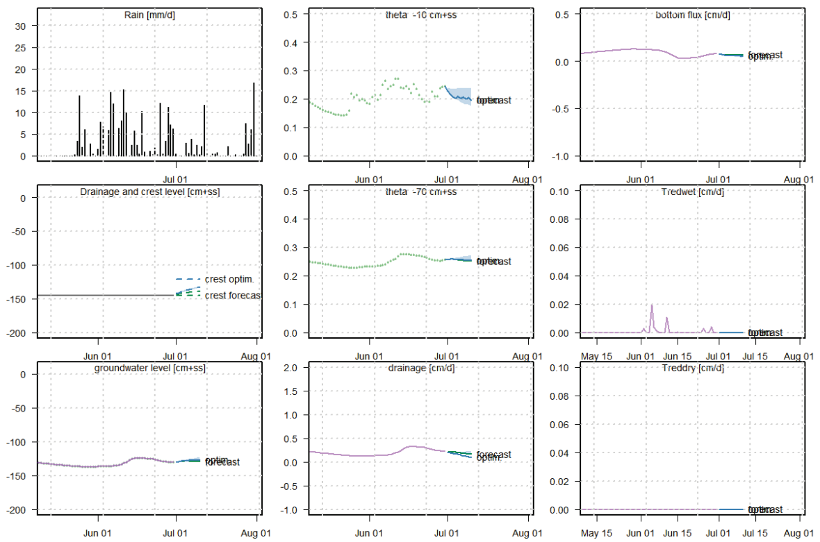
Figure 21: Example of forecast and optimization of the crest level for conditions with superfluous drainage. In order to limit the future drainage flux (forecast), the crest level needs to be increased (crest optim., see also Figure 21).
