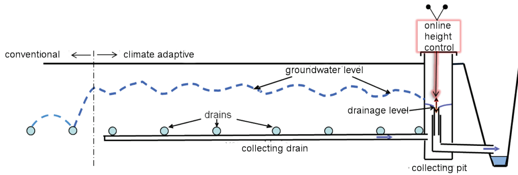
Figure 1: Climate Adaptive Drainage (CAD) system: subsurface drains, connected to a closed collecting drain, ending up in a collecting pit with drainage basis control unit, with outlet to the surface water system.
