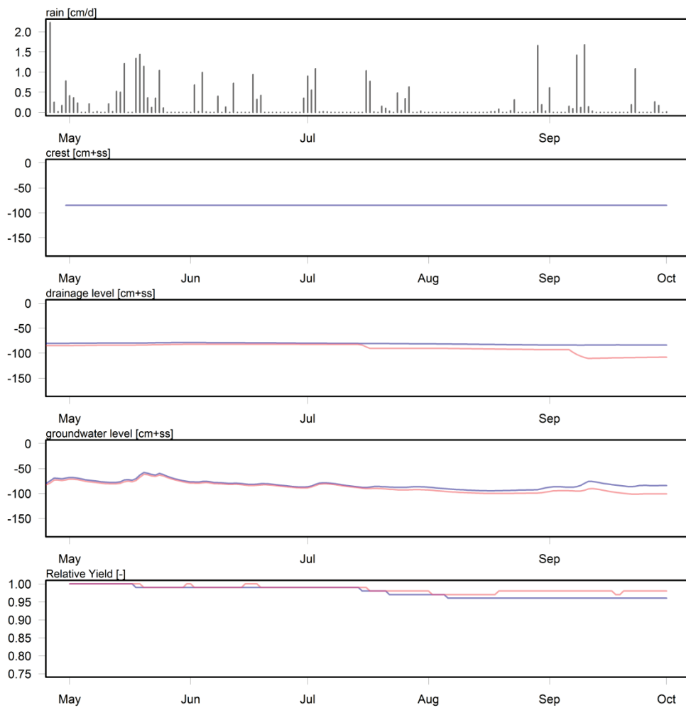
Figure 10: Example simulations for dynamic CAD crest management (red) vs. a fixed crest (blue) for the year 2003 (dry).
