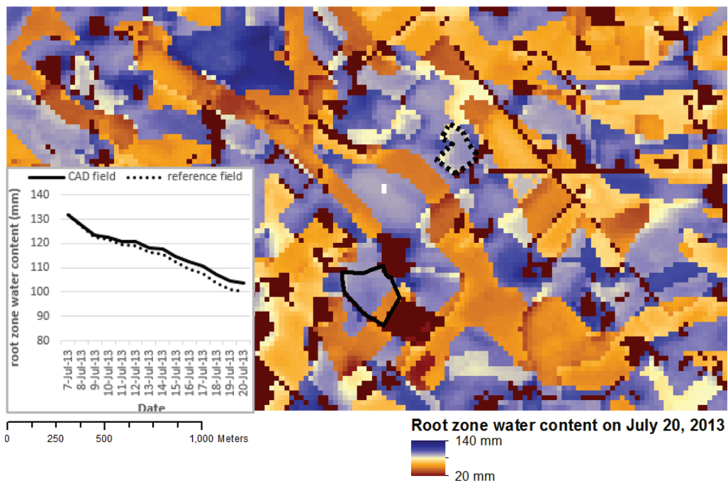
Figure 15: Spatial and temporal visualization of differences in root zone soil water content between the Haaksbergen CAD test site and a reference maize field without CAD. Locations of the CAD field and reference field are indicated on the map by the solid and dashed black lines respectively.
