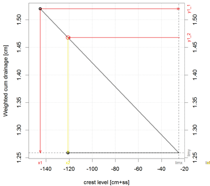
Figure 19: Optimization routine, if \Sigma weighted positive Drainage > limit. First, the drainage flux (limy, see y-axis) at the highest possible crest level (limx, see x-axis) is calculated with SWAP. Then, the next crest level is derived by i) calculate y-value by a fraction of the difference between y1\_1 (the current weighted cumulative drainage) and limy: y1\_2 = limy + factor * abs(y1\_1 - limy) , ii) calculate next x value from a linear relationship between (x1, y1\_1) and (x2, y(1\_2)) , iii) run swap with this x value, which gives a new yn\_1 value. This procedure is repeated until: abs(y1\_1 - limy) \leq factor * abs(limy) (i.e. very small relative difference with lowest possible value) or abs(y1\_1) \leq abs(limy.accept) (i.e. smaller than accepted value) or sum(str.out, "Tredwet") * myweights > Tredwet.cum.accept (i.e. weighted cumulative Tredwet larger than accepted weighted value or x1\_2 < minx or x1\_2 > maxx ) (i.e. next estimate of crest level below lowest or above highest possible crest level) or nrow(it.out) > 100 (i.e. too many iterations).
