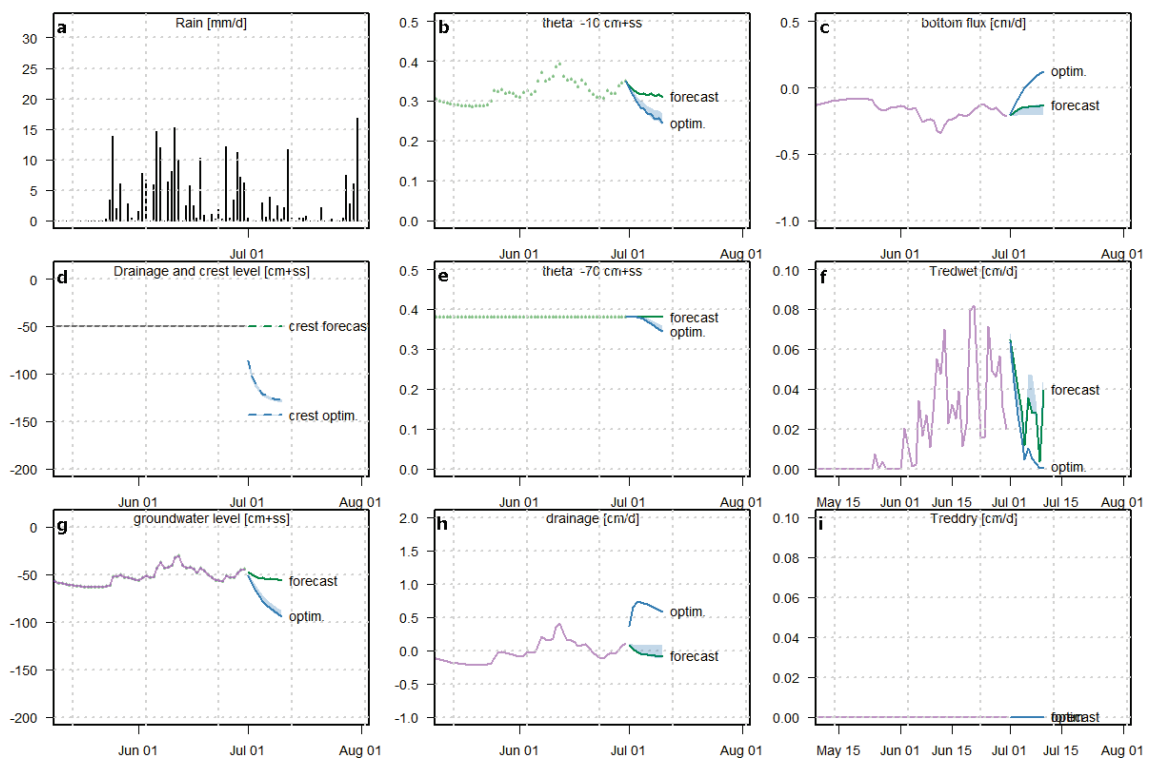
Figure 5: Example of forecast and optimization of the crest level for wet conditions. In order to limit future oxygen stress (f: Tredwet, forecast), the crest level needs to be lowered (d: crest optim.). This will increase the drainage flux (h), lower the groundwater level (g) and soil moisture content (b: theta), and limit oxygen stress (f: Tredwet).
