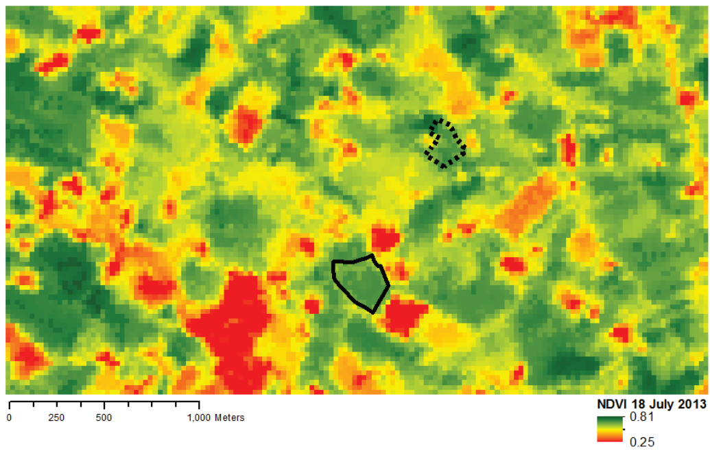
Figure 14: Regional-scale high-resolution NDVI on July 18, 2013. Locations of the CAD field and reference field without CAD are indicated on the map by the solid and dashed black lines respectively.
