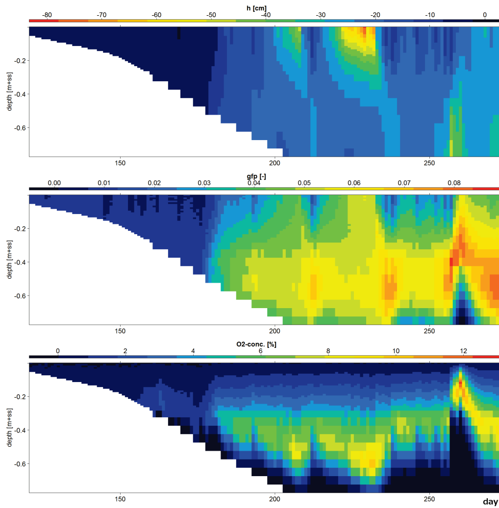
Figure 9: Differences of soil water pressure head ( h ), gas filled porosity ( gfp ) and oxygen concentration ( O_2\text{-conc} ) in the root zone for the growing season of 1998, for simulations with a fixed and with a dynamic crest (Figure 8). Given values = results dynamic crest - results fixed crest. The root depth increases during the growing season, with a maximum depth of -0.7\text{m+s.s.} around day 200; this explains the white area in the figures.
