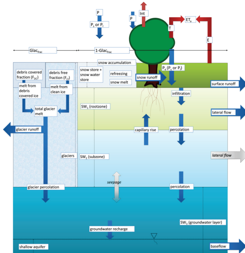
Figure 6: SPHY model concept. Several of these concepts, such as the glacio-hydrological module of the model, are optional and switched off in the current application ( www.sphy.nl ).
