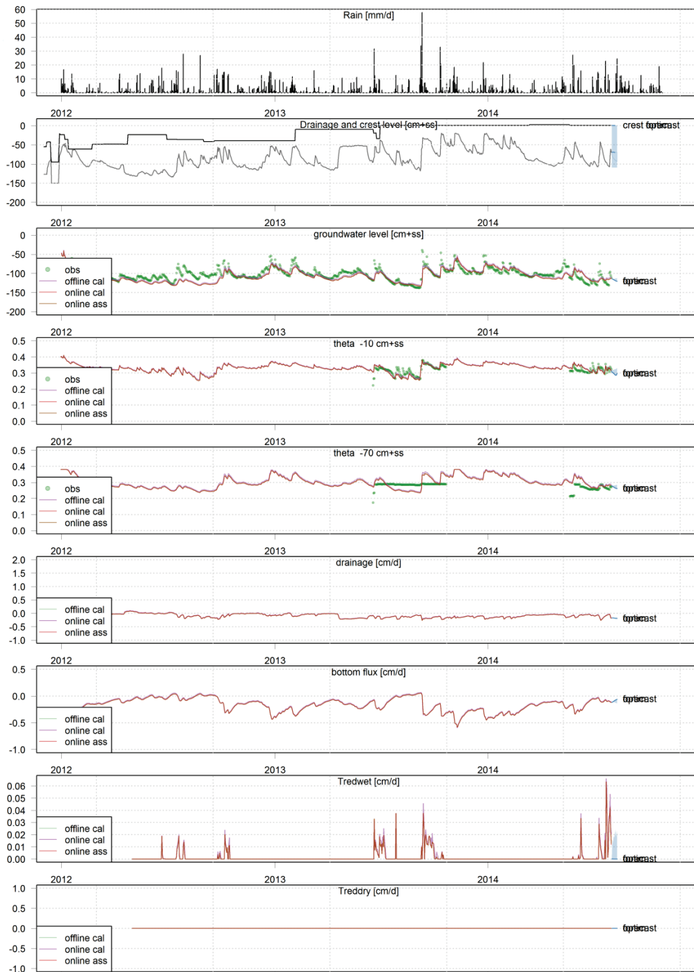
Figure 11: Example of measured and simulated (after calibration and assimilation) groundwater levels and soil moisture conditions, and simulated plant stresses for the Haaksbergen CAD test site. Please note that for this example, calibration and assimilation runs provide almost similar results (lines overlap). Theta = soil moisture content, Tredwet = transpiration reduction due to oxygen stress, Treddry = transpiration reduction due to drought stress. See also Figure 12, which zooms in on the 10-day forecast and optimization runs.
