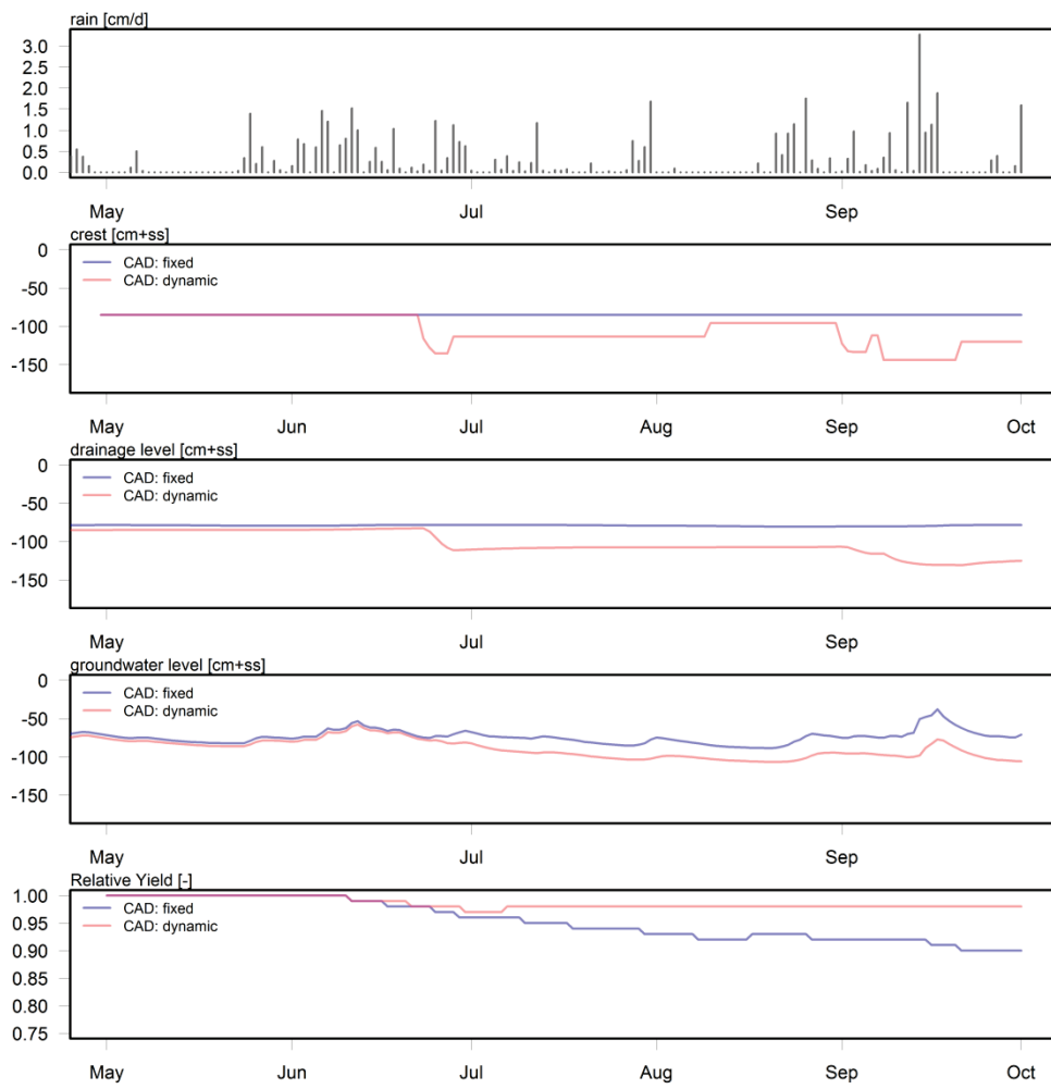
Figure 8: Example simulations for dynamic CAD crest management (red) vs. a fixed crest (blue) for the year 1998 (wet).
