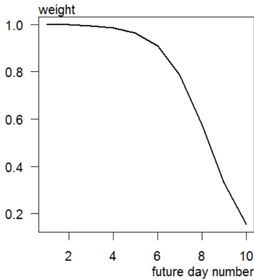
Figure 17: Weight function used in the calculation of the weighted cumulative potential transpiration and weighted cumulative drainage. The shape of the function can easily be altered in R_swap_pest.R. With the given sigmoid function, the forecast conditions for 10 days in the future, get a lower weight in the optimization scheme than conditions of the next day.
